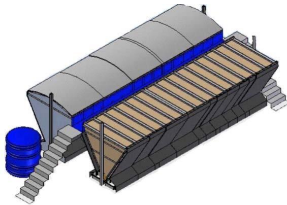
Industrial Design. Above has a capacity of 6000kg/wk, configured into 30 cells. This Design is Infinitely Expandable
